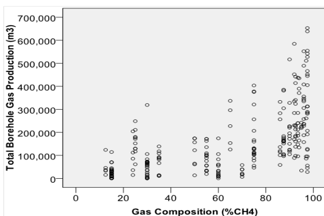
Figure 11(A) – Total gas production relative to gas composition
