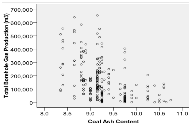
Figure 7(A) – Total gas production relative to coal ash content
