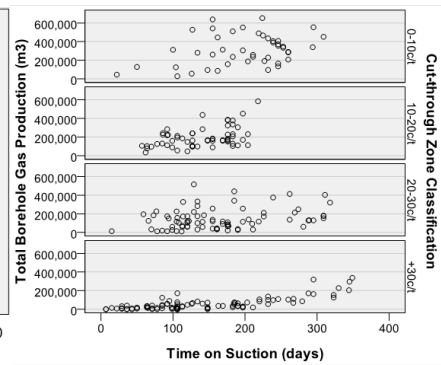
Figure 5(C) – Total gas production relative to drainage time grouped based on drill site location
