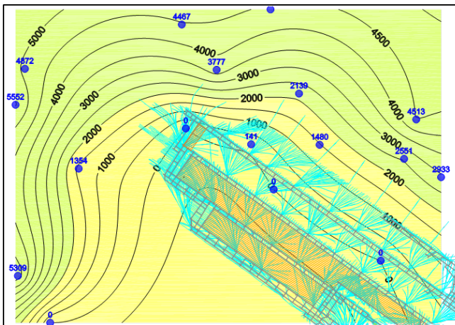
Figure 14(A) – Seam pressure gradient (kPa) relative to advancing mine workings and gas drainage – Feb. 2007
