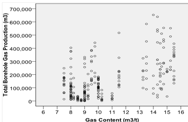
Figure 10(A) – Total gas production relative to gas content
