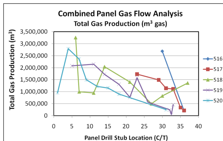
Figure 2 – Total drill stub gas production relative to panel drill stub location
