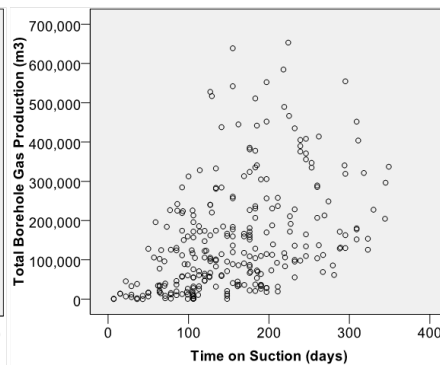
Figure 5(B) – Total gas production relative to drainage time
