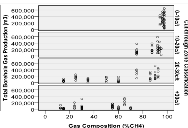
Figure 11(B) – Total gas production relative to gas composition grouped based on drill site location
