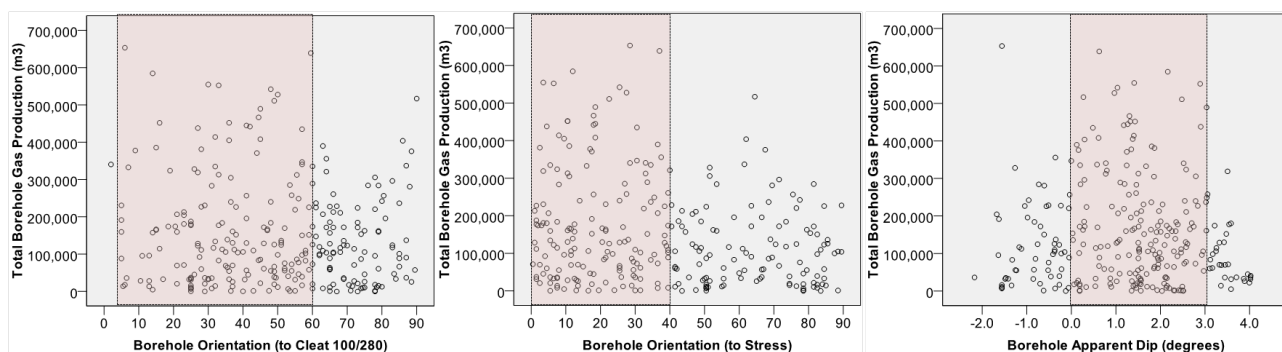
Figure 4(A) – Total gas production relative to borehole orientation to cleat (100/280°)
