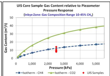
Figure 15(C) – In situ gas condition in deeply undersaturated, CO 2 rich inbye zone
