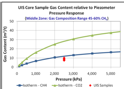
Figure 15(B) – In situ gas condition in moderately undersaturated, mixed gas (CH 4 /CO 2 ) middle zone
