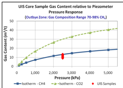
Figure 15(A) – In situ gas condition in slightly undersaturated, CH 4 rich outbye zone
