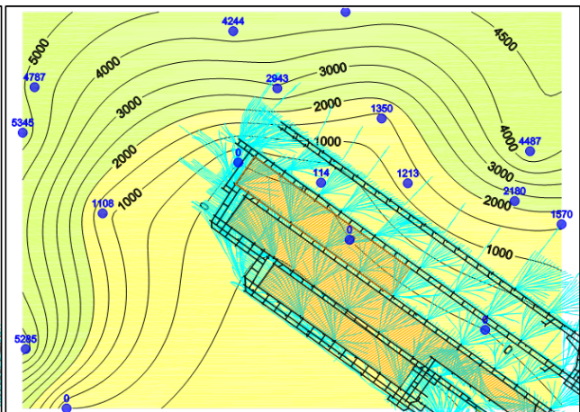
Figure 14(B) – Seam pressure gradient (kPa) relative to advancing mine workings and gas drainage – Sep. 2007
