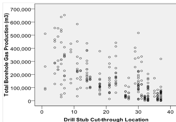
Figure 3 – Total gas production relative to borehole location along panel
