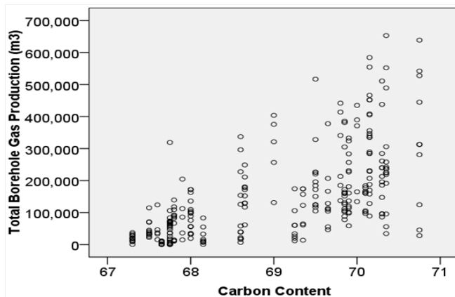
Figure 6(A) – Total gas production relative to carbon content
